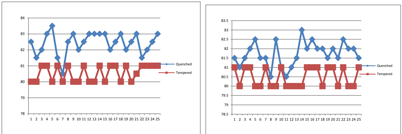
Fig no.6 Hardness variation after quenching and tempering also, before and after modification
