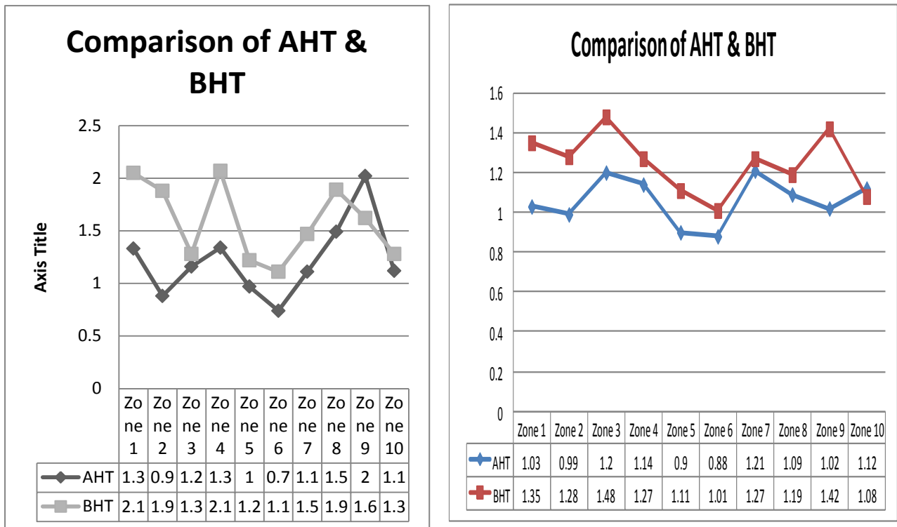
Fig no. 4 Comparison trend of AHT & BHT and also, before & after modification of guide vane area
